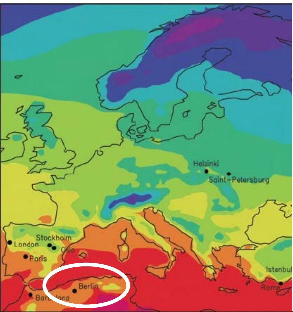
Hadley Center model, HadRM3H , Climat Emission scenario SRES/A2
